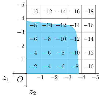
FIGURE 0.2. F_\ell(X_\Omega, \mathbb{K})_T for a convex toric domain.
